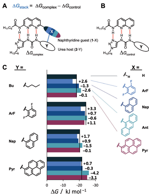
Figure 1. A), B) Supramolecular complexes used to measure aromatic stacking interactions in solution. C) Experimental complexation free energies determined in 5% (v/v) CD 3 CN in CDCl 3 at 298 K. Dissected experimental stacking free energies \Delta G_{\text{stack}} are displayed in kJ mol -1 to the right of the bar for each X–Y contact, as determined using the equation shown in (A). Errors in \Delta G are <1.1 kJ mol -1 in all cases (twice the standard error). All data and errors are provided in the Supporting Information.
