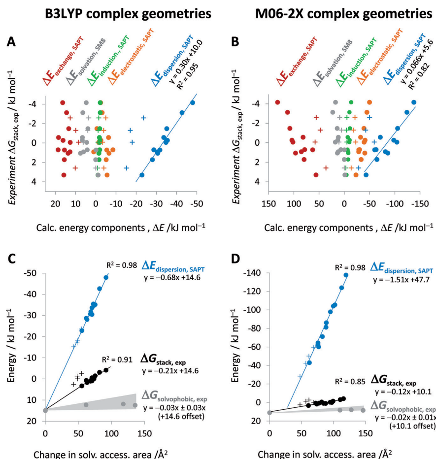
Figure 2. A), B) Experimental stacking free energies versus partitioned energy components for stacked X–Y geometries calculated using DF-SAPT0 with the aug-cc-pVDZ' basis set. Solvation energy changes in chloroform calculated using SM8 are also shown. The dispersion energy component correlated most strongly with the experimental data. Circles correspond to Y = aryl group while crosses are Y = n -butyl. C), D) Correlation of experimental stacking free energies (black) and calculated SAPT0 dispersion energies (blue) against the change in solvent accessible area on association of X and Y in the model complexes. Solvophobic contributions were estimated from independent measurements of solvent effects on aromatic stacking interactions previously reported by Cubberley and Iverson (gray) (Supporting Information, Figure S9). [14a,d] The geometries of each X–Y interaction used in the SAPT0, SM8 and solvent accessible area calculations were determined from minimized structures of the H-bonded complexes using either the B3LYP or M06-2X level of theory and the 6-31G* basis set as indicated. The intercepts of solvophobic contributions are offset to match those of the experimental data to ease comparison of the gradients. Error bars in the experimental energies are < 1.1 \text{ kJ mol}^{-1} in all cases. Correlation coefficients are only shown where R^2 > 0.76 .
